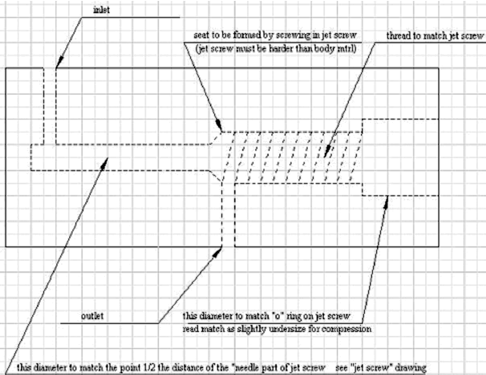
Valve Body (Brass)
